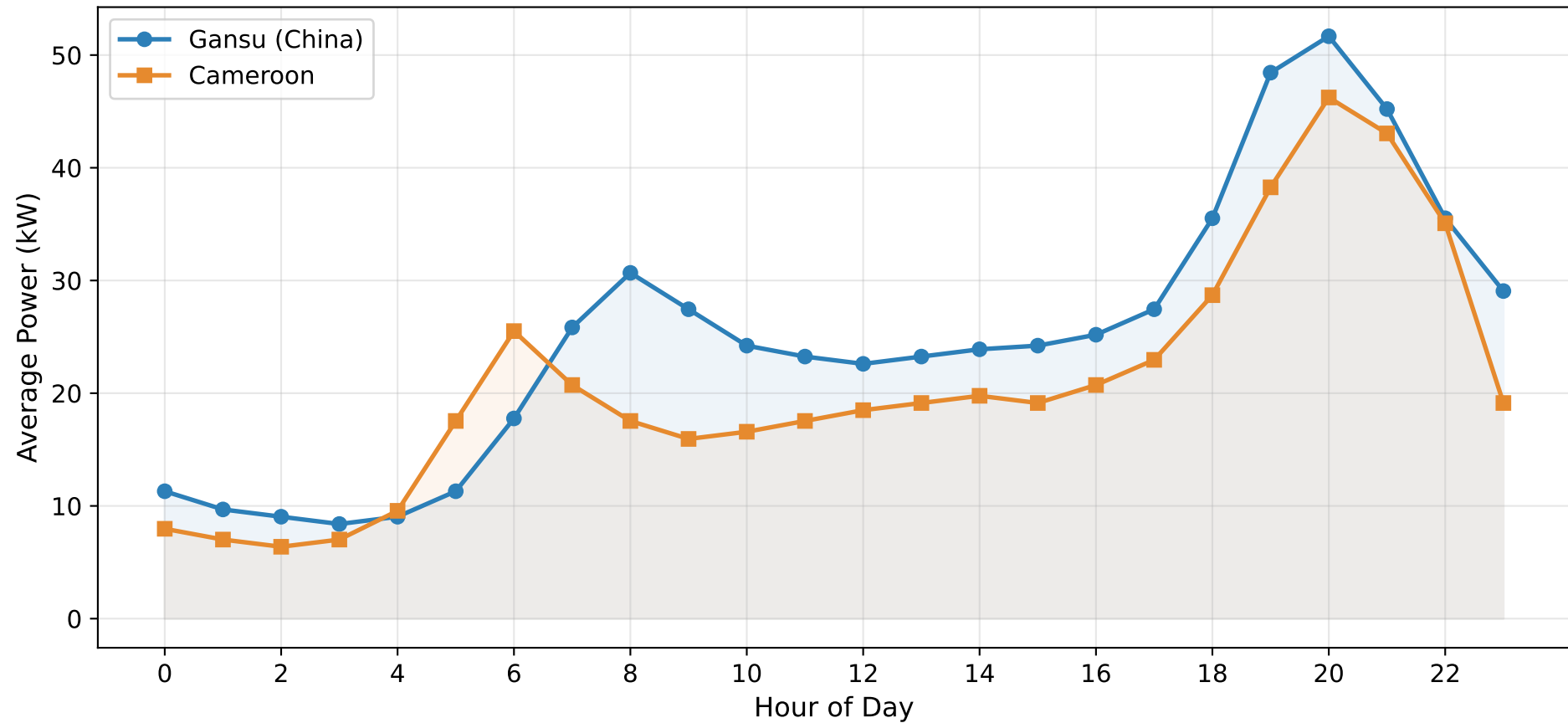
Typical Daily Load Profile (200 households)
