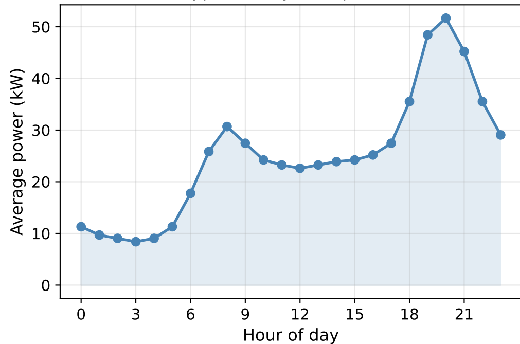
Typical daily load profile
