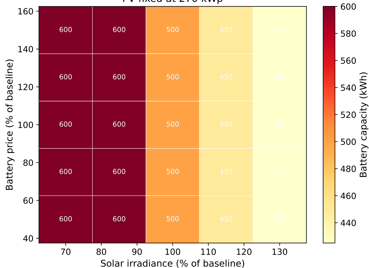
Required Battery Capacity (kWh) for LPSP \leq 5\% PV fixed at 270 kWp
