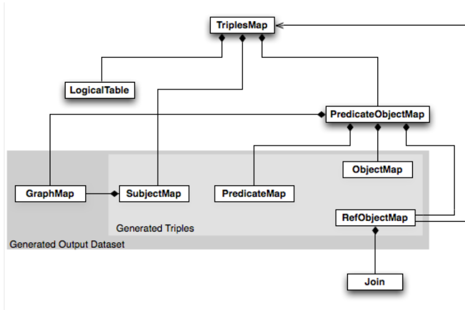
Figure 1: An overview of R2RML
