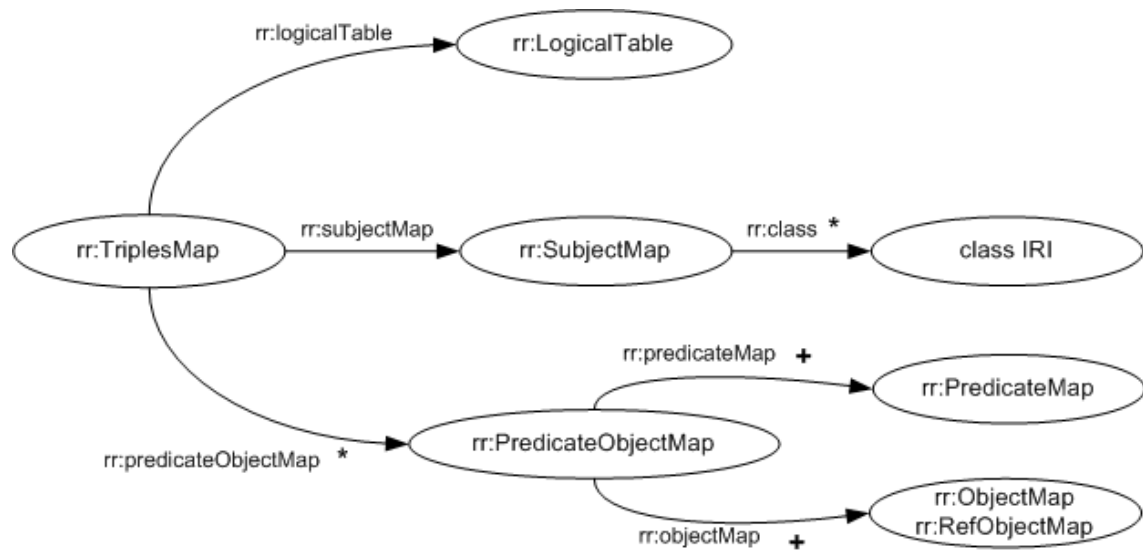
Figure 3: The properties of triples maps
