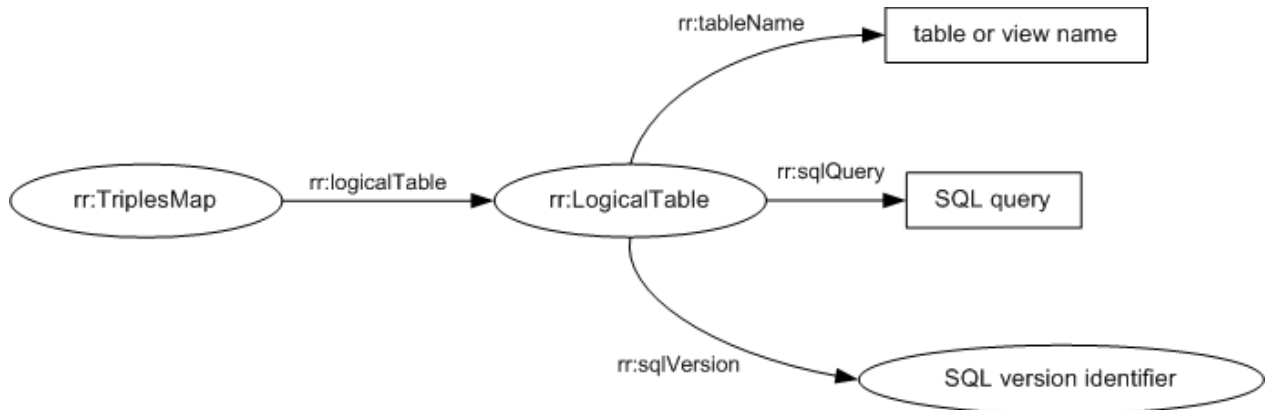
Figure 2: The properties of logical tables
