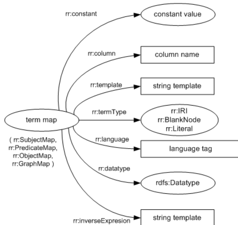
Figure 4: The properties of term maps
