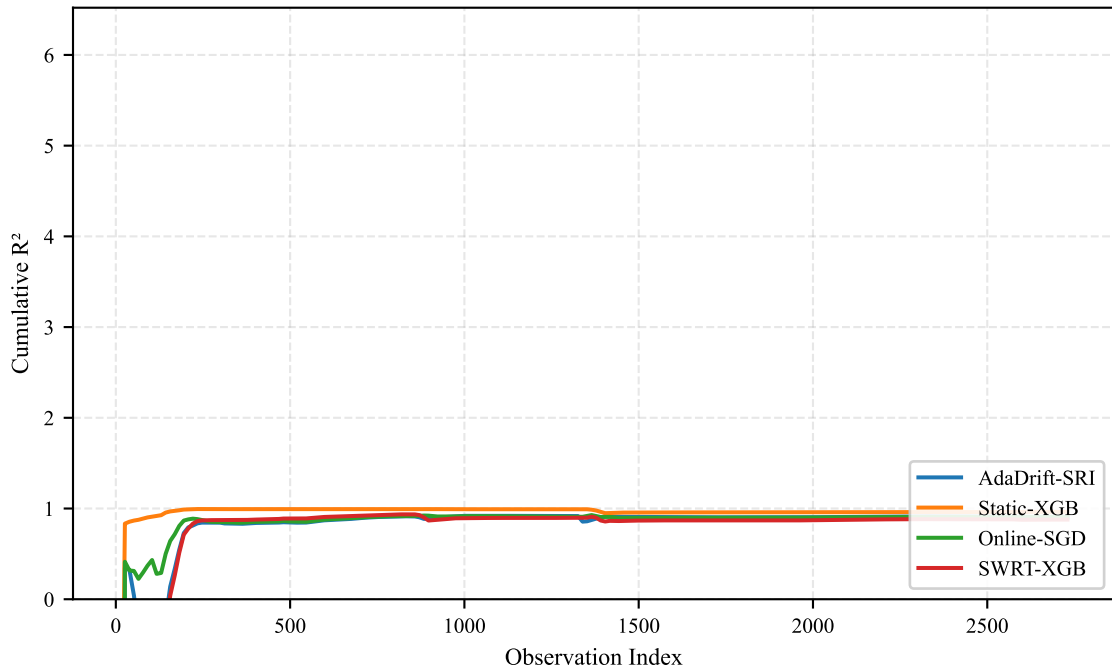
Fig. 1: Cumulative R^2 Score Progression
