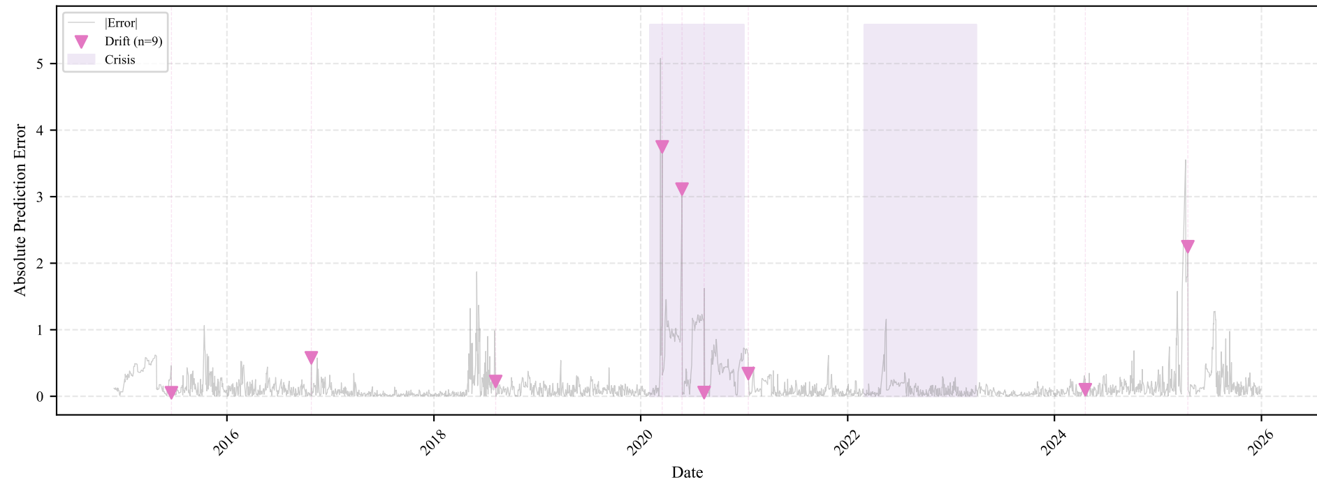
Fig. 4: Drift Detection Timeline — 9 Drifts Detected
