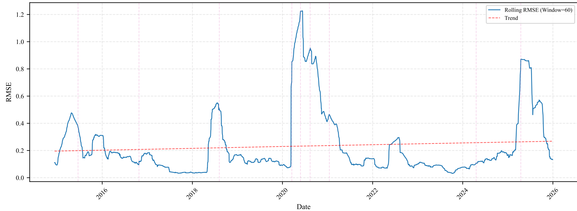
Fig. 5: Rolling RMSE Performance Monitoring
