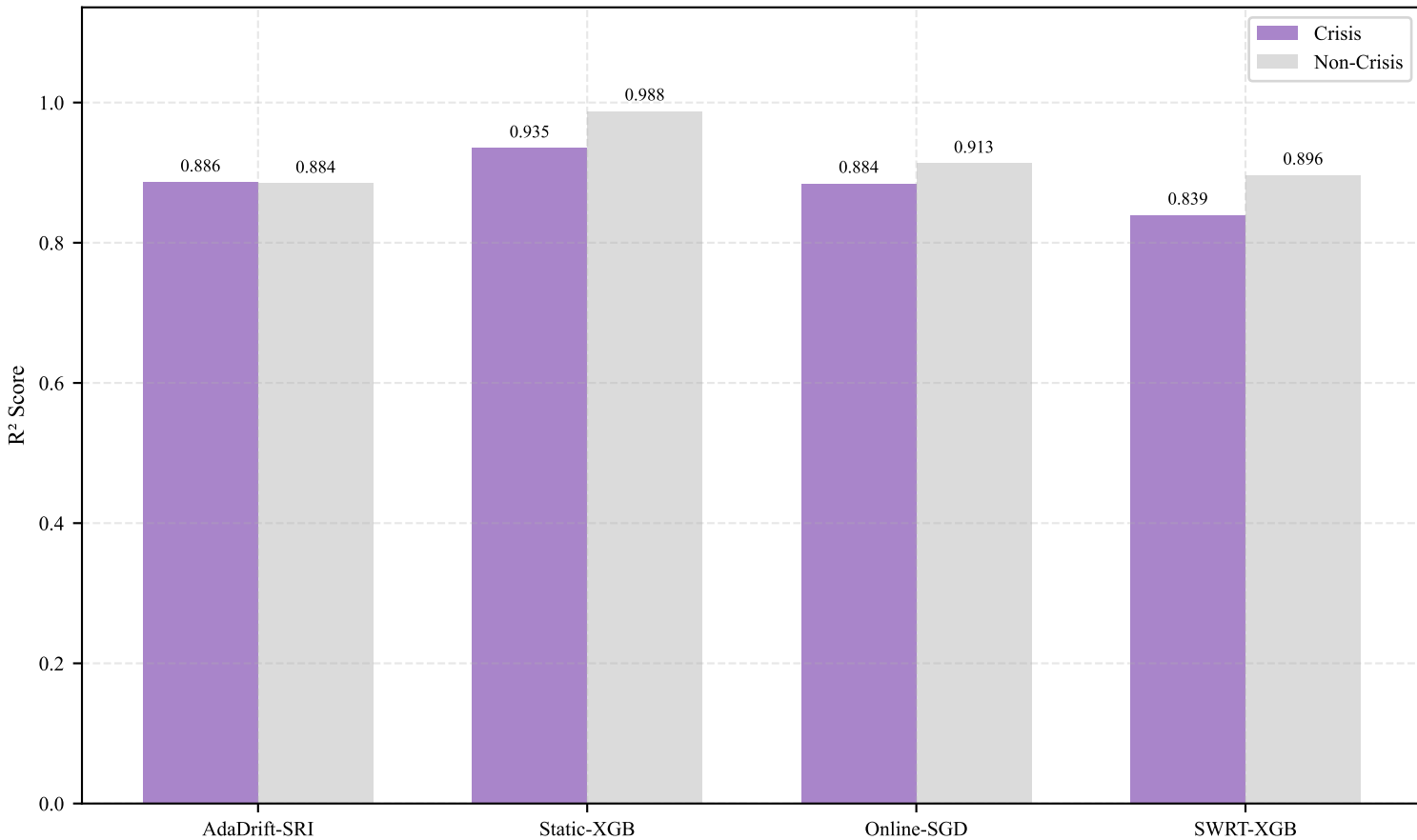
Fig. 6: Model Performance — Crisis vs Non-Crisis Periods
