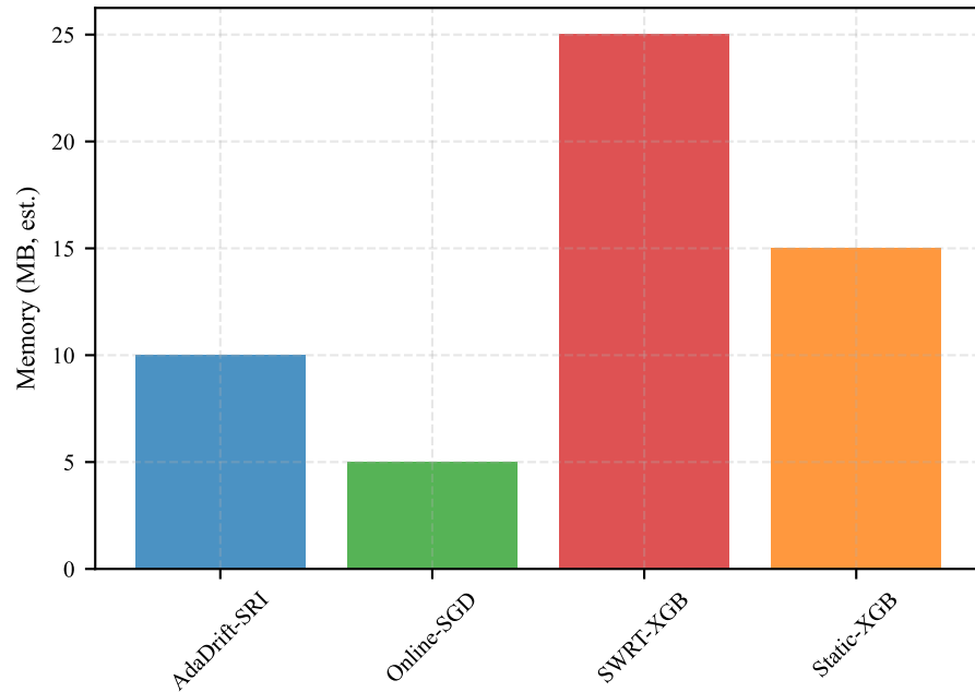
Memory Usage
