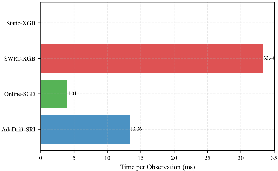
Processing Speed
