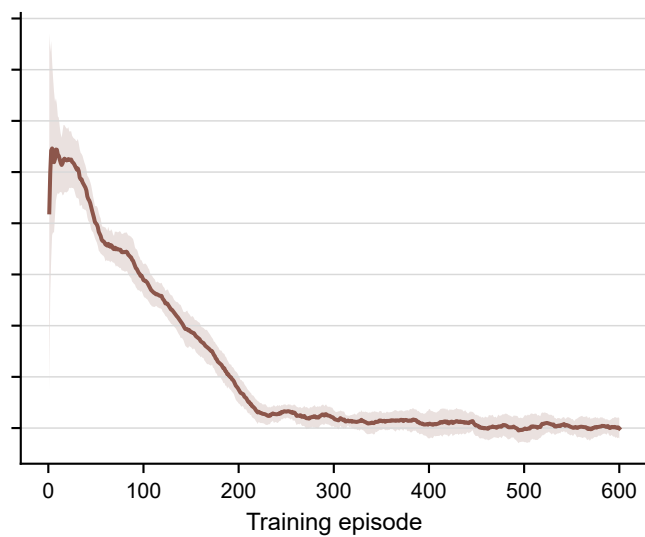
Double + centered
