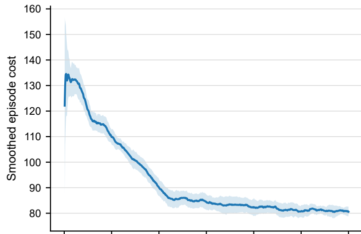
Centered full-action
