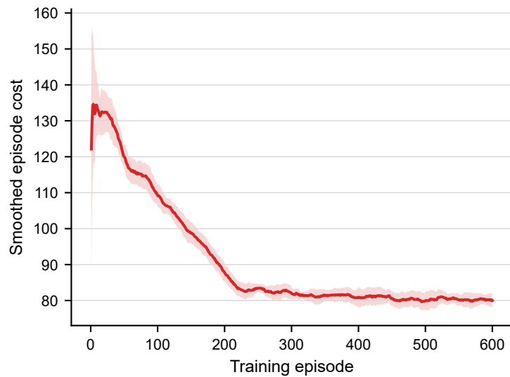
Centered full-action
