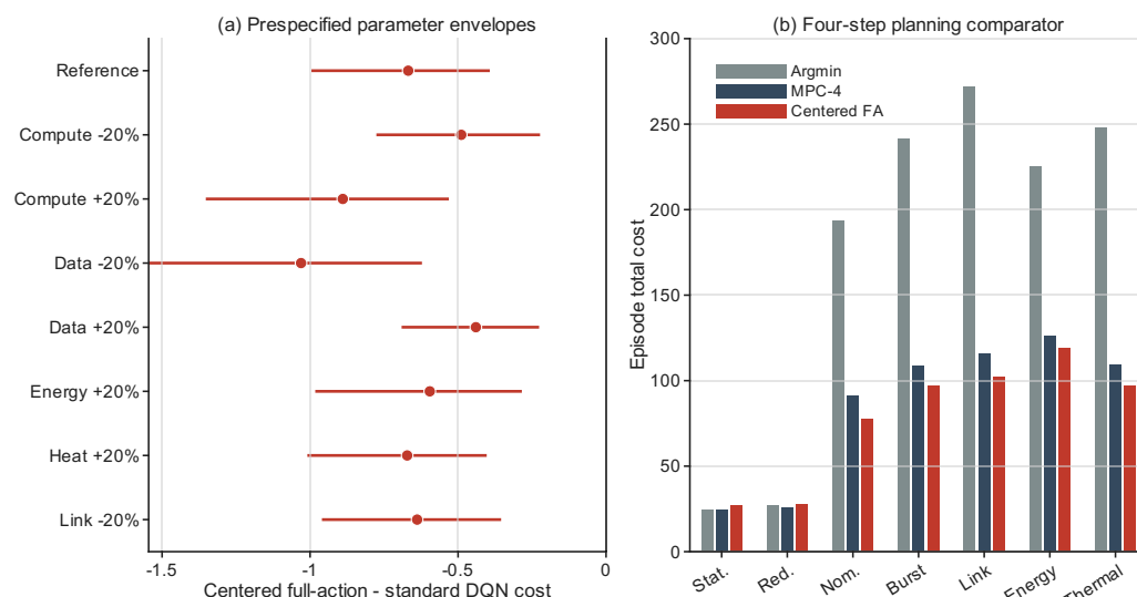
Figure 7. Parameter sensitivity and planning boundary. (a) Mean paired differences between centered full-action and standard DQN with 95% paired bootstrap intervals. (b) Immediate, four-step rolling, and learned scheduling across coupling and stress regimes.
