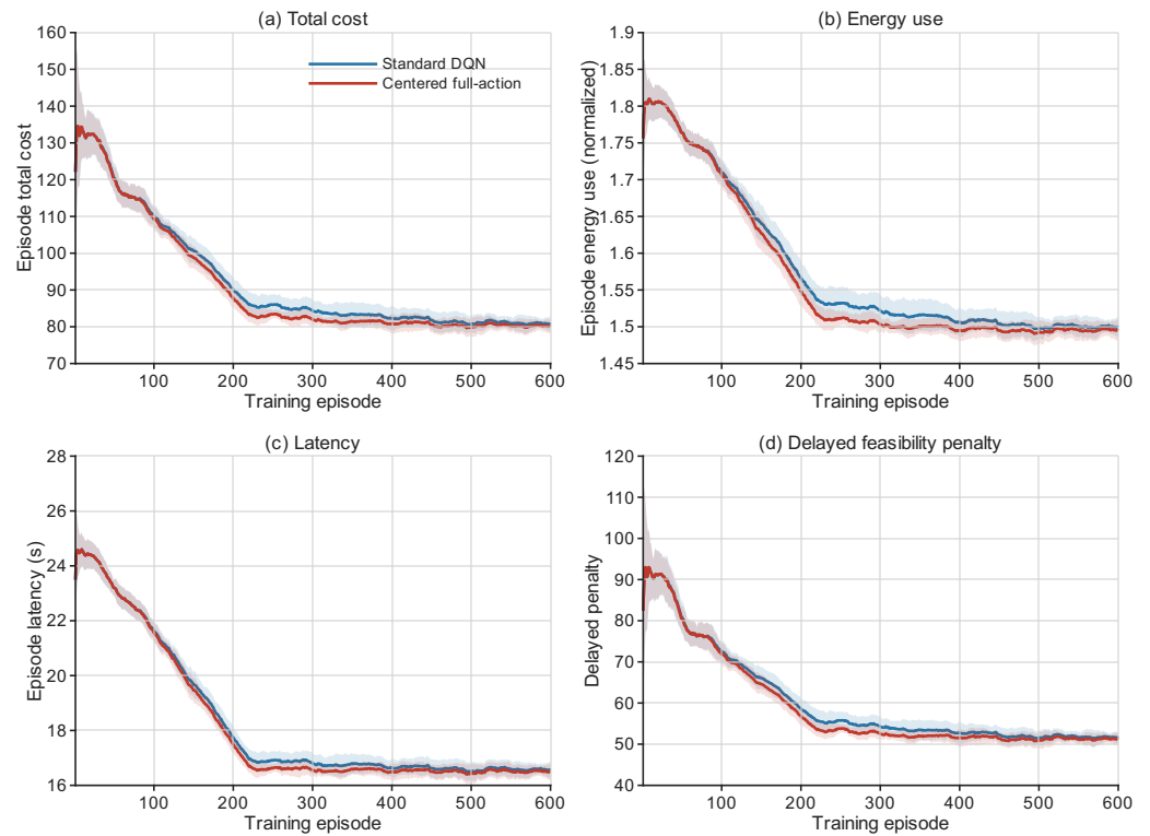
Figure 6. Representative training diagnostics for standard DQN and the centered full-action DQN variant. Lines are means across 20 model seeds after a causal 25-episode moving average; shaded regions are \pm 1 SD. Curves describe the training distribution and are not used as independent test observations or evidence for the whole DQN family.
