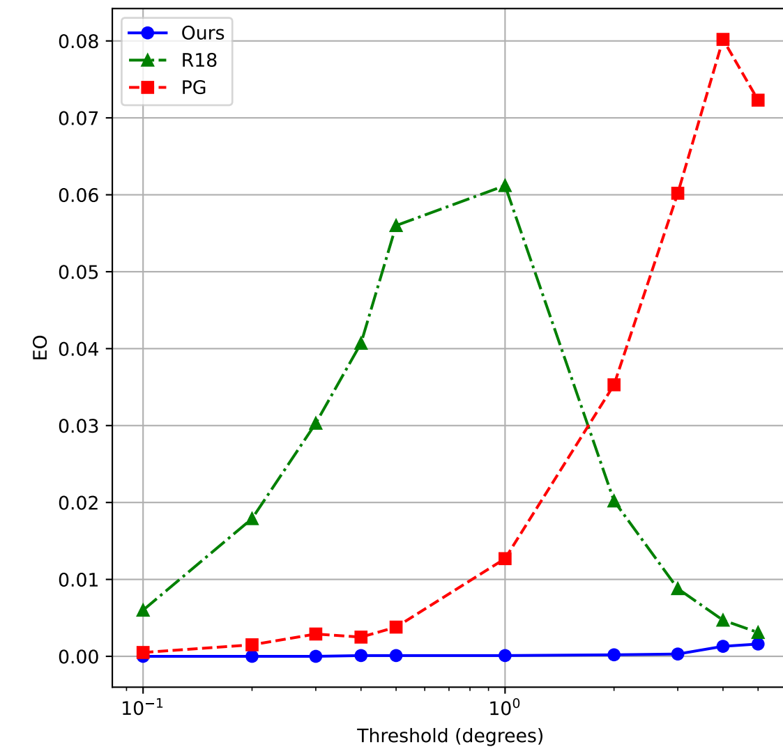
XGaze → XGaze
