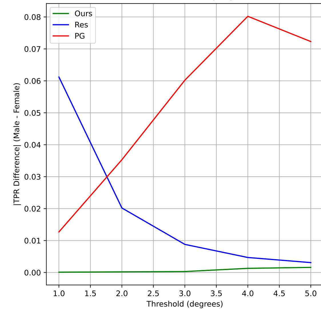
XGaze → XGaze (1-5)
