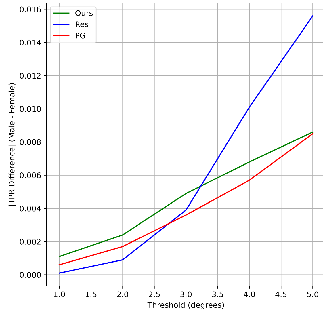
XGaze → XGaze (1-5)
