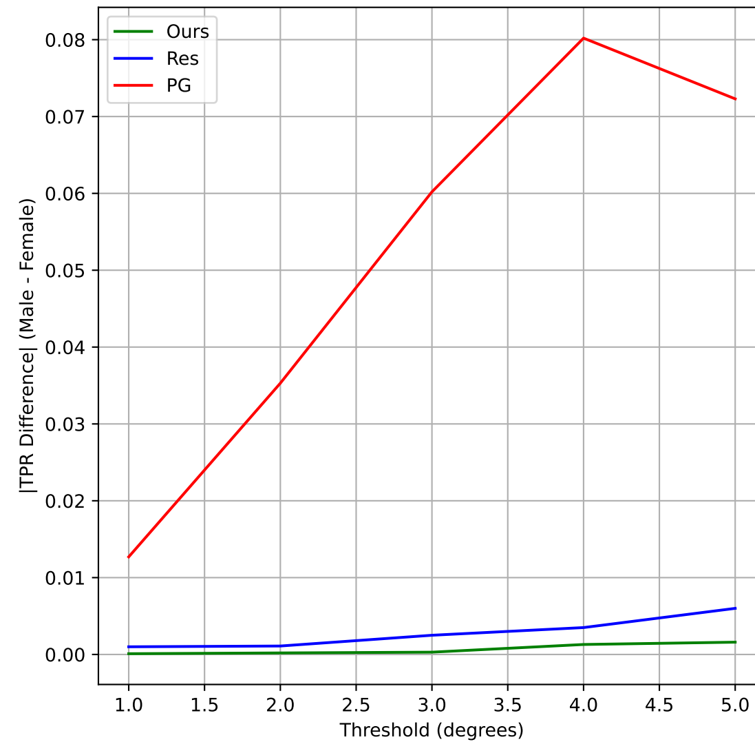
MP11 → MP11 (1-5)
