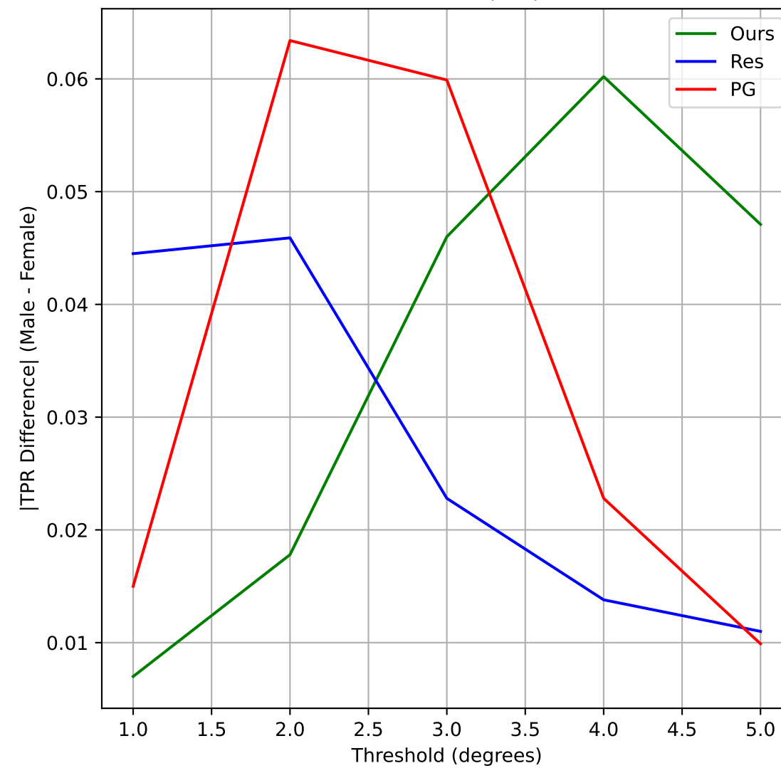
MP11 → MP11 (1-5)
