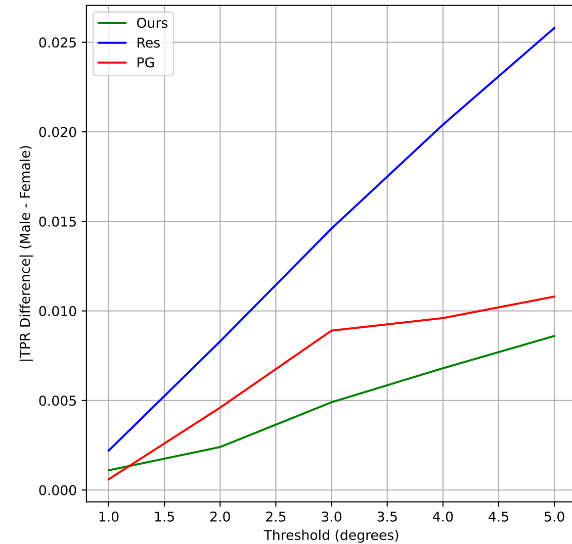
MP11 → XGaze (1-5)
