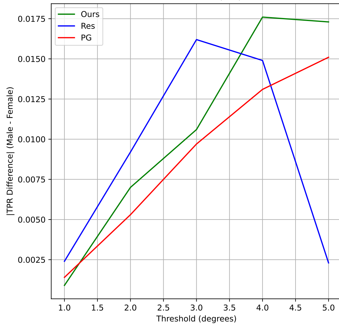
MP11 → XGaze (1-5)
