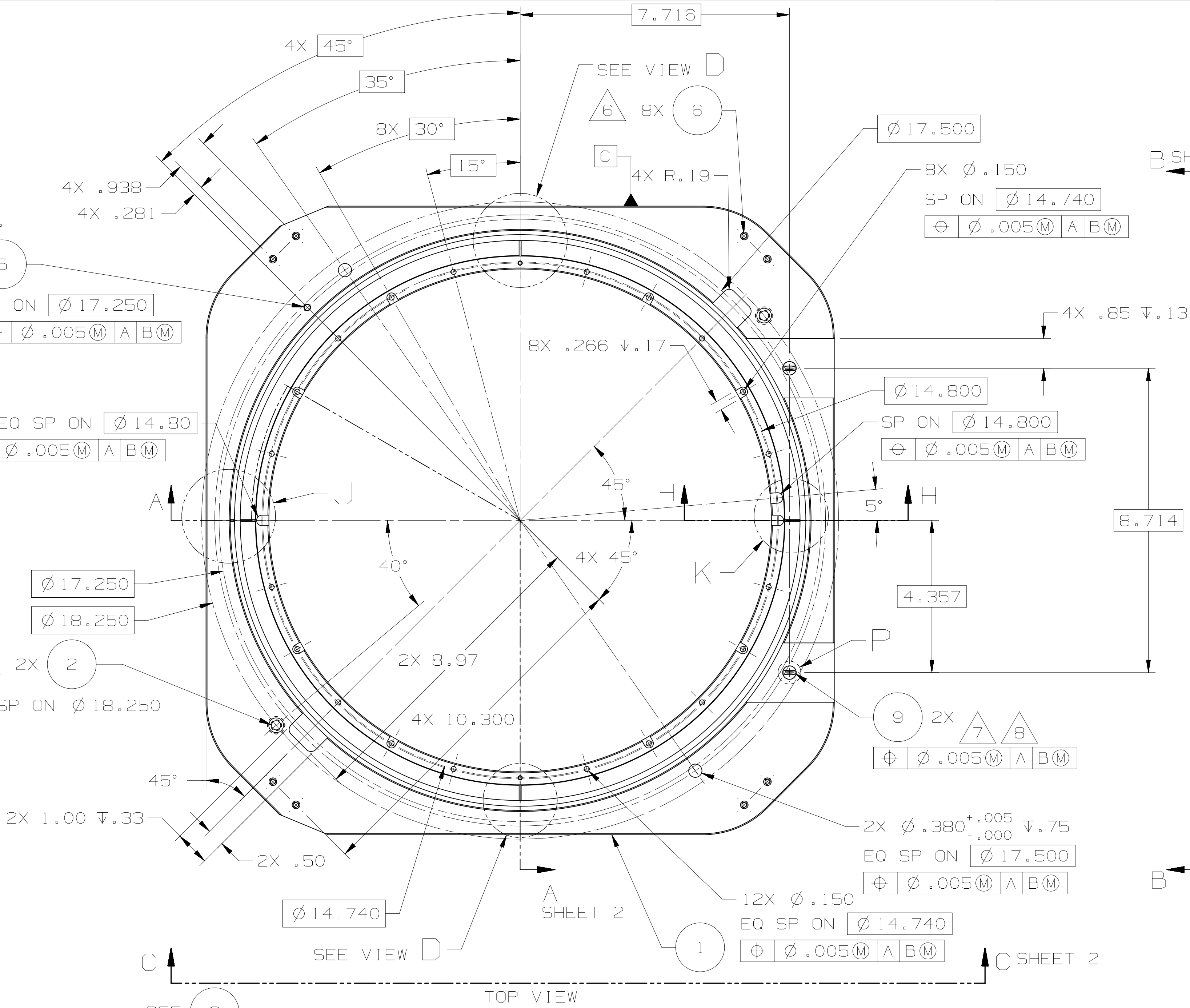
TOP VIEW
