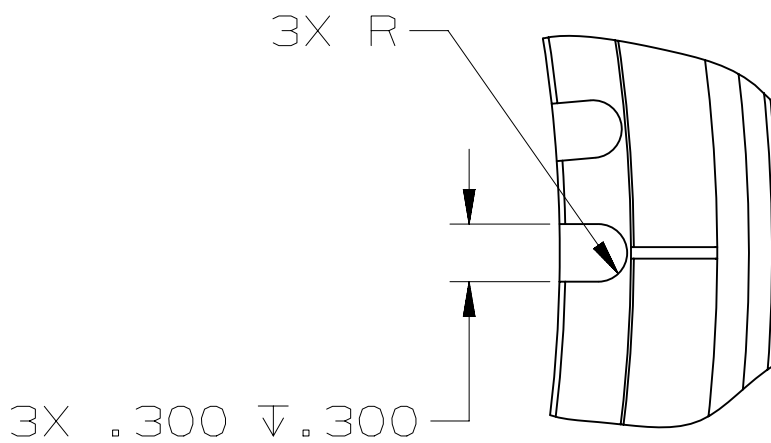
DETAIL K
