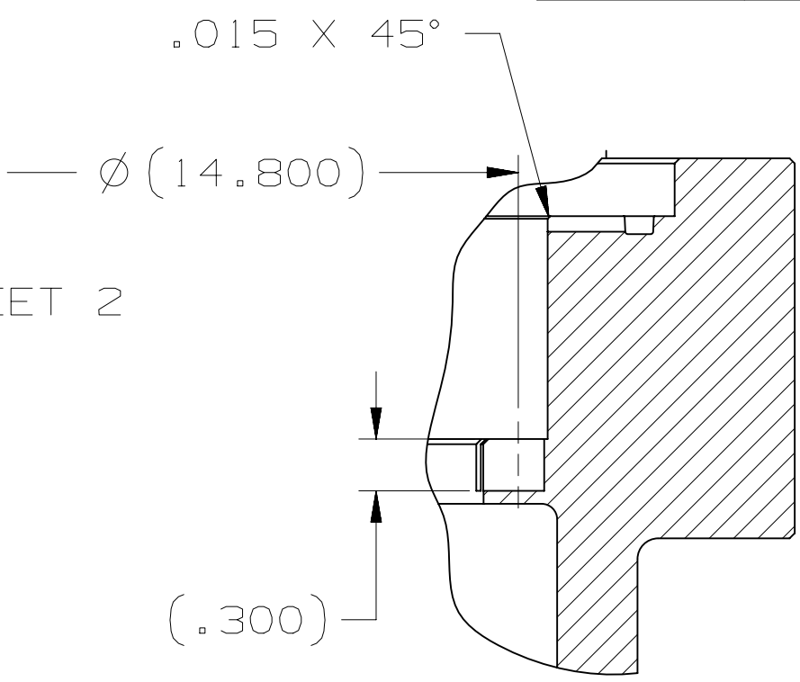
SECTION H-H
