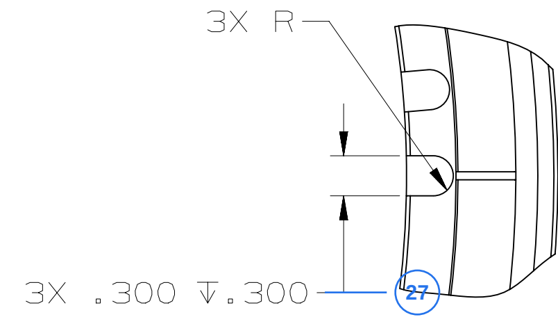
DETAIL K
