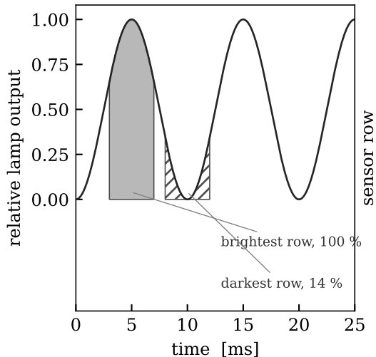
(a) lamp on a 50 Hz supply, output period 10 ms two 4.0 ms exposure windows
