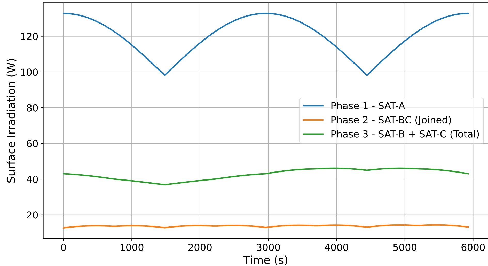
Global Phase Comparison - Orbital Angle 94°
