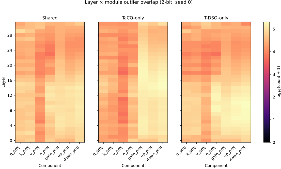
Figure 2: Layer \times module outlier decomposition (2-bit, seed 0): shared, TaCQ-only, and T-DSO-only kept weights.
