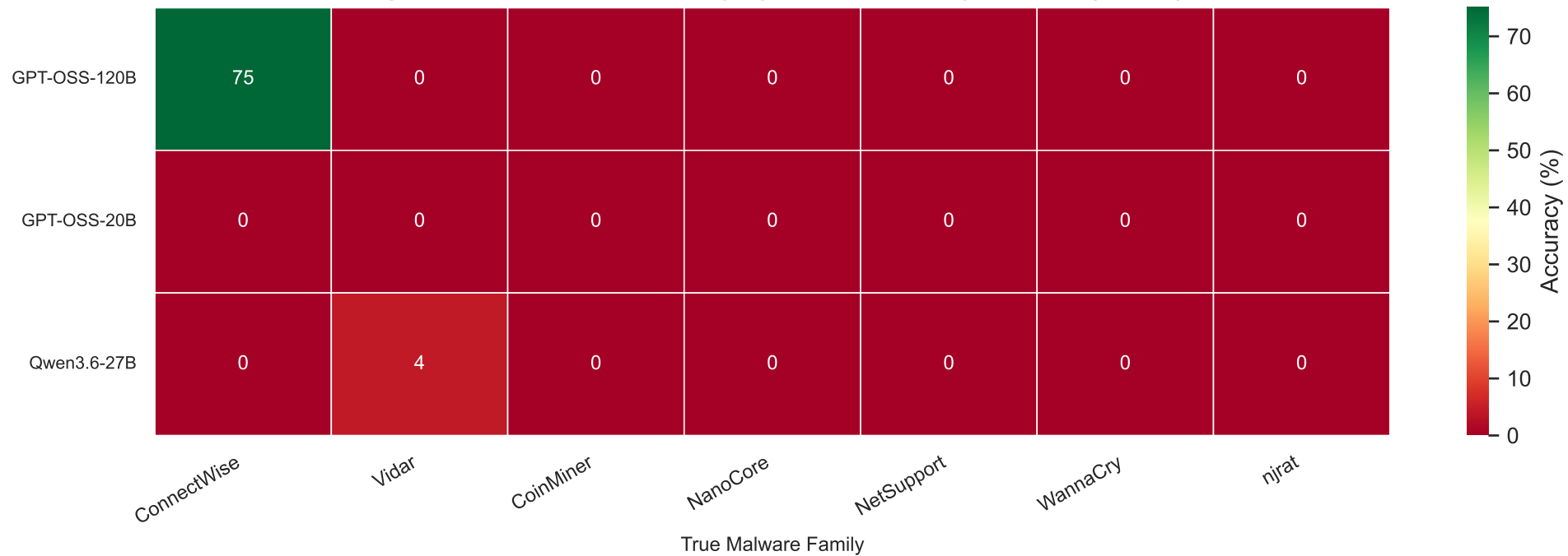
Fig. -- Classification Accuracy by Malware Family x Model (N=504)
