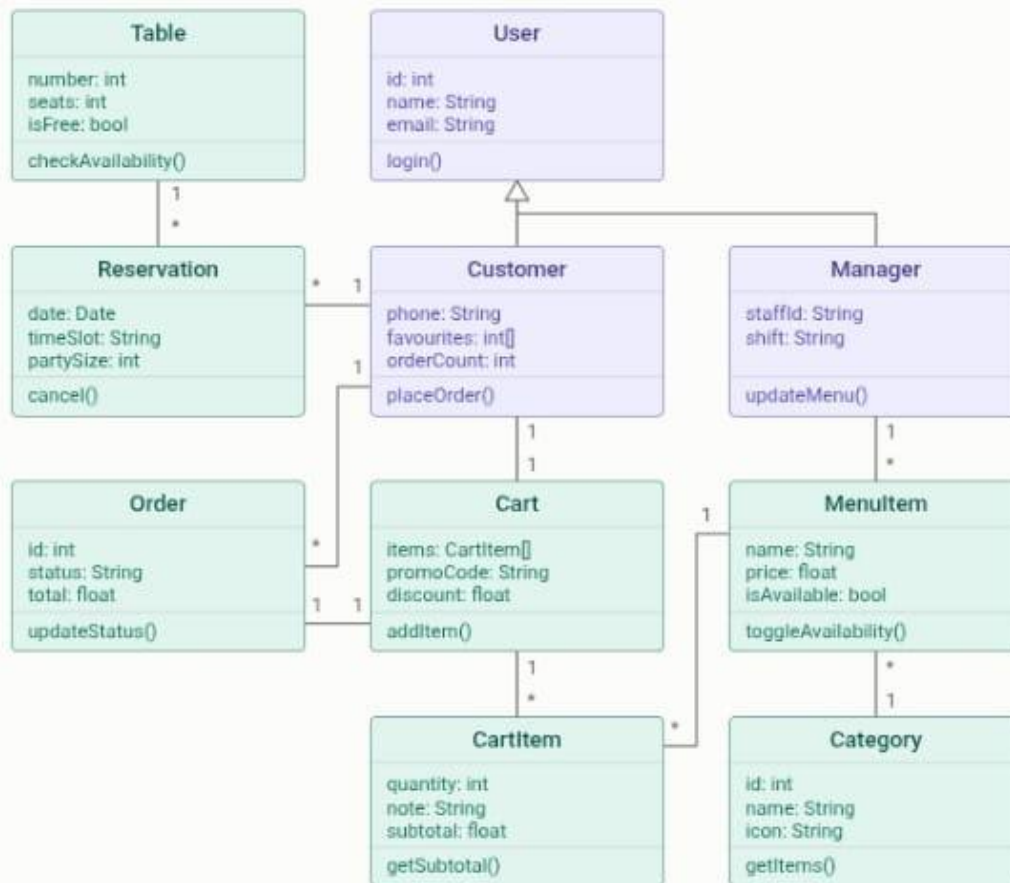
Class diagram of the restaurant app mvp
