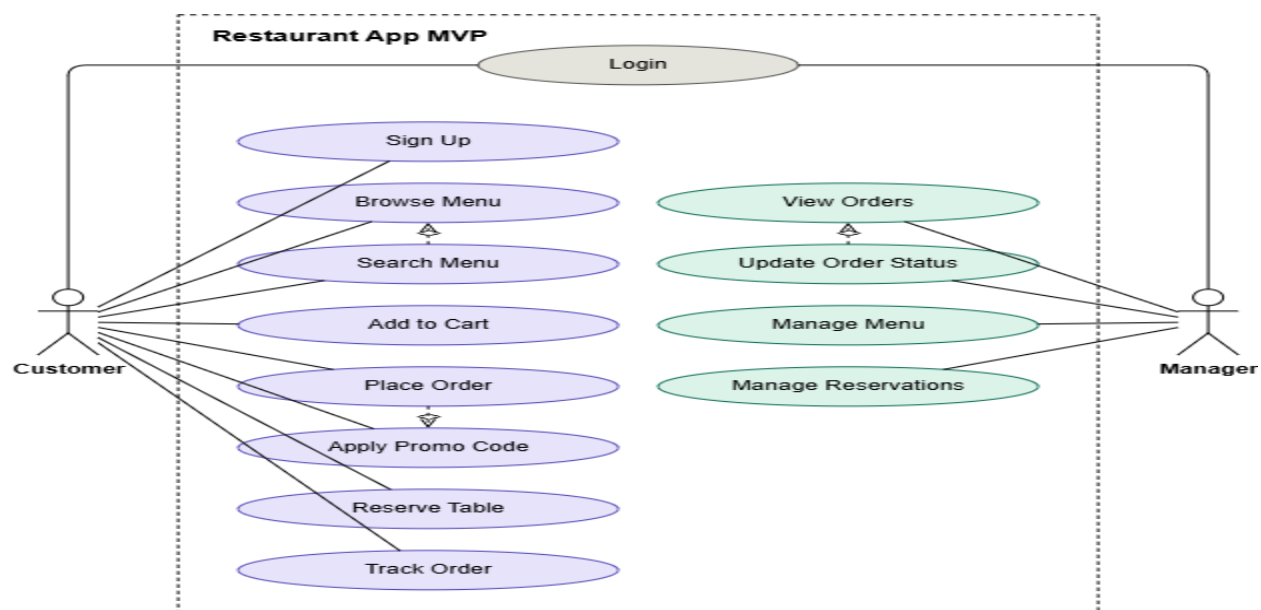
Usecase diagram of the restaurant app mvp
