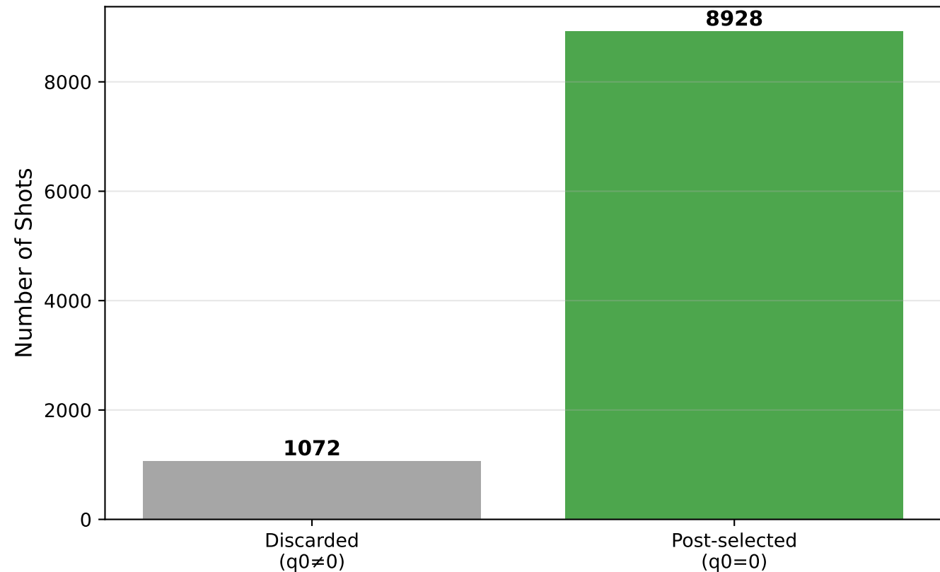
Post-Selection Statistics (Total shots: 10000)
