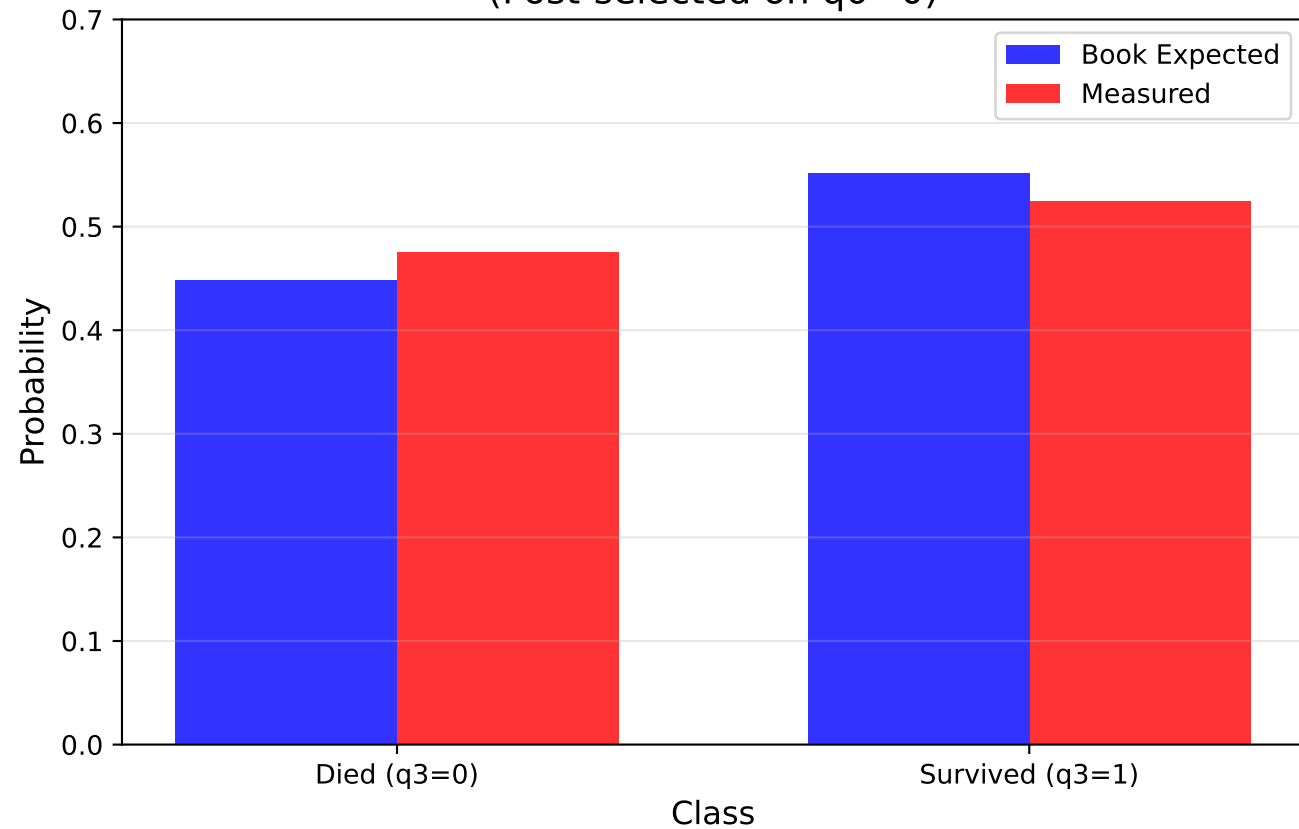
Classification Probabilities (Post-selected on q_0=0 )
