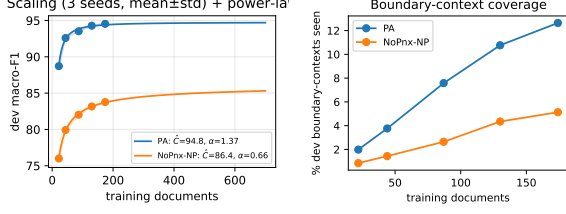
Figure 2: Left: dev F_1 vs. training-set size (3 seeds, mean \pm std) with power-law fits \hat{C} - a n^{-\alpha} extrapolated to 700 docs. PA is at its asymptote ( \alpha=1.37 ); NoPnx-NP scales slowly toward a lower, still-unreached asymptote ( \alpha=0.66 ). Right: fraction of dev boundary contexts seen in training—only 5% for NoPnx-NP. Both locate the ceiling in data quantity.
