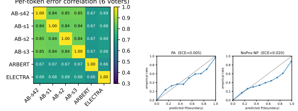
Figure 3: Left: per-token error correlation across the six voters (mean off-diagonal 0.74). Right: reliability diagrams; the ensemble is well calibrated (ECE 0.005/0.020).
