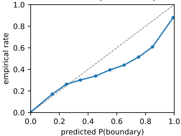
NoPnx-NP (ECE=0.020)
