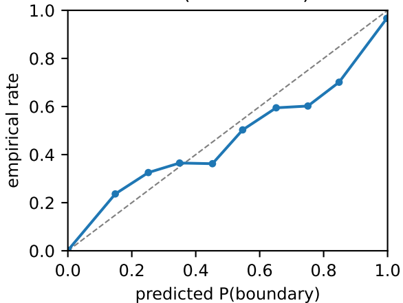
PA (ECE=0.005)
