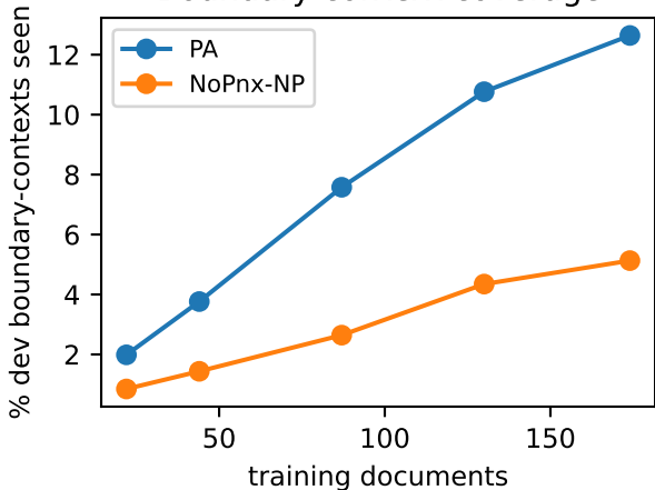
Boundary-context coverage
