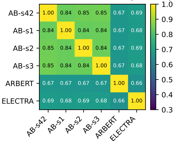
Per-token error correlation (6 voters)
