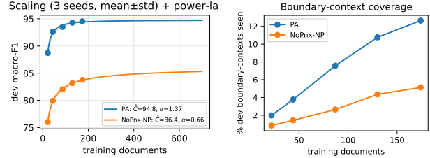
Figure 2: Left: dev F_1 vs. training-set size (3 seeds, mean±std) with power-law fits \hat{C} = a n^{-\alpha} extrapolated to 700 docs. PA is at its asymptote ( \alpha=1.37 ); NoPnx-NP scales slowly toward a lower, still-unreached asymptote ( \alpha=0.66 ). Right: fraction of dev boundary contexts seen in training—only 5% for NoPnx-NP. Both locate the ceiling in data quantity.
