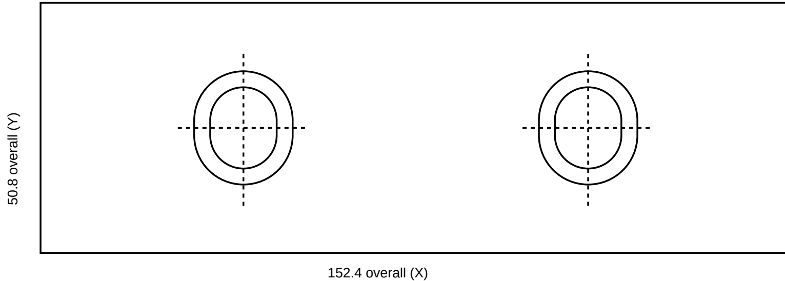
TOP VIEW - slot long axes parallel to Y
