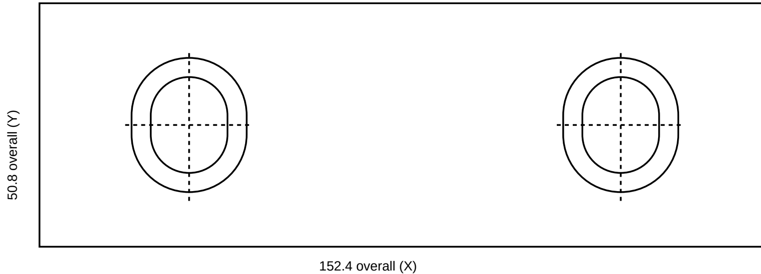
TOP VIEW - slot long axes parallel to Y
