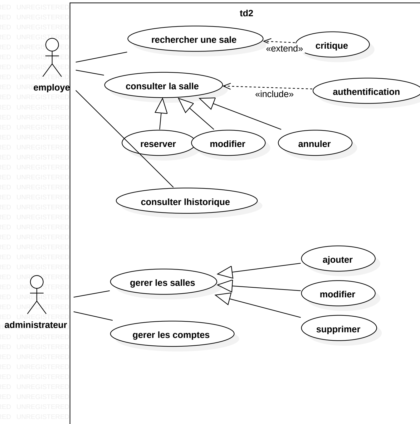
Model1::UseCaseDiagram1
