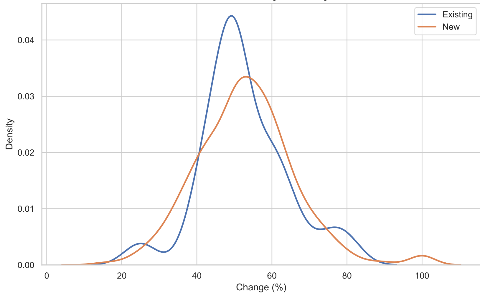
Distribution of Change Percentage
