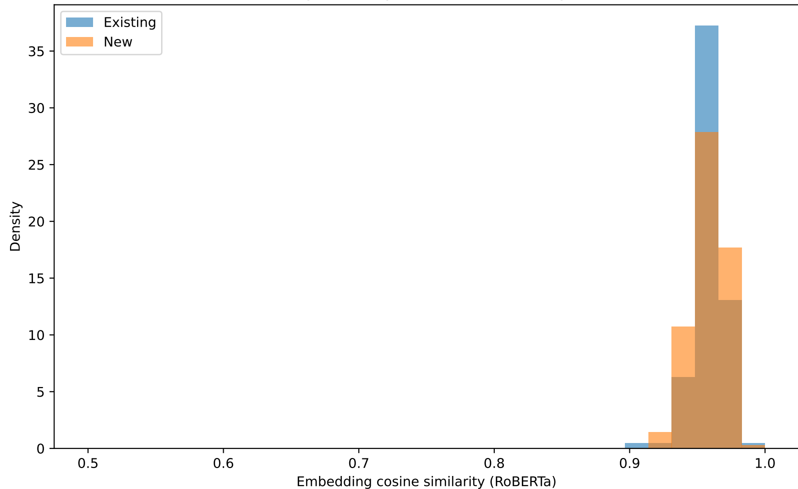
Embedding Similarity Distribution: Existing vs New
