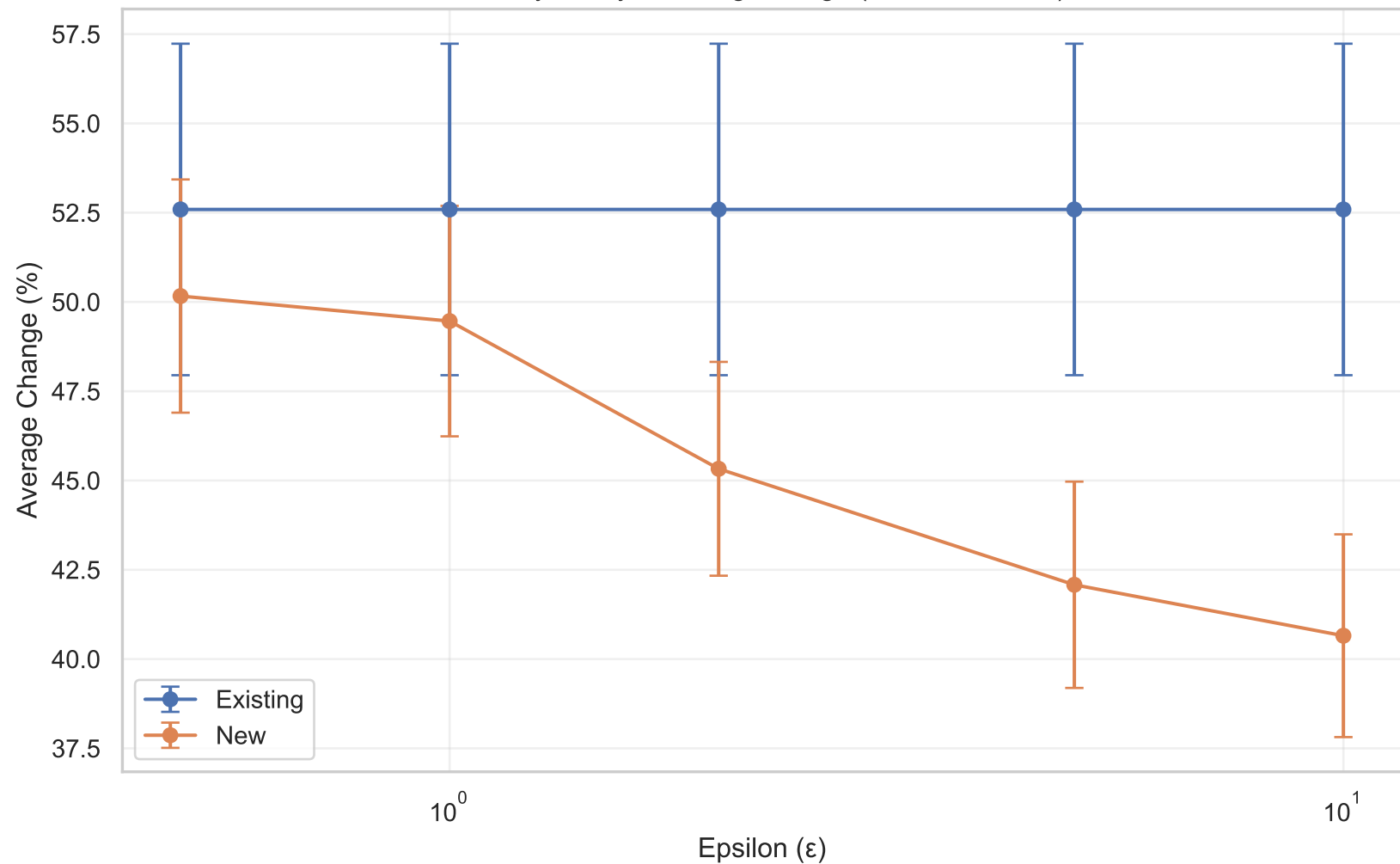
Privacy–Utility: \epsilon vs Avg Change (mean \pm 95% CI)
