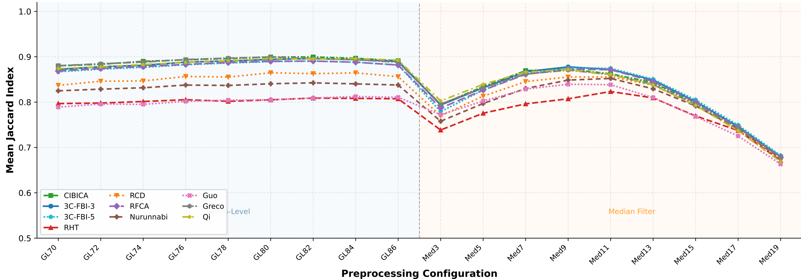
Experiment A — Mean Jaccard Index across 18 Preprocessing Configurations (144 clinical frames, 10 methods)
