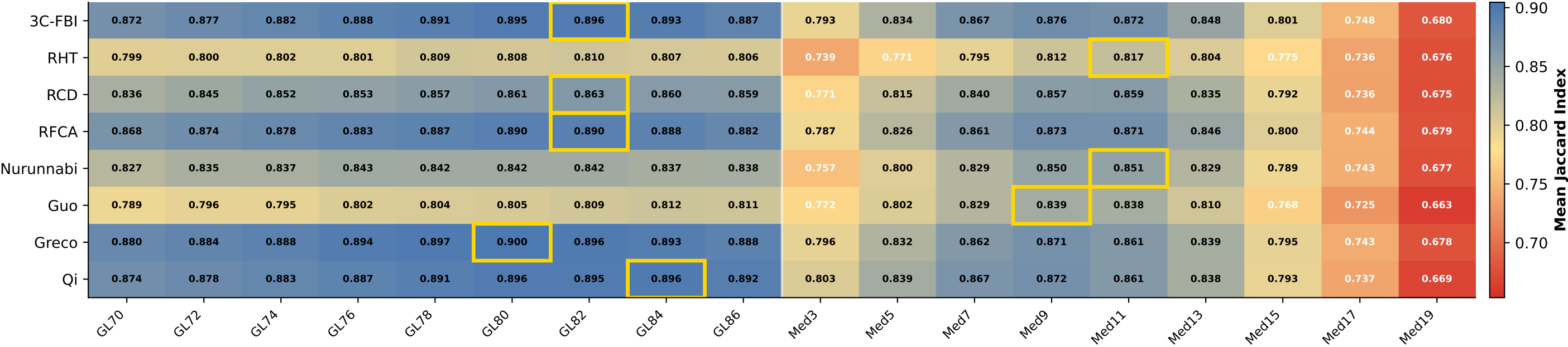
Experiment A — Jaccard Index Heatmap (Methods × Preprocessing Configs) Gold border = best config per method
