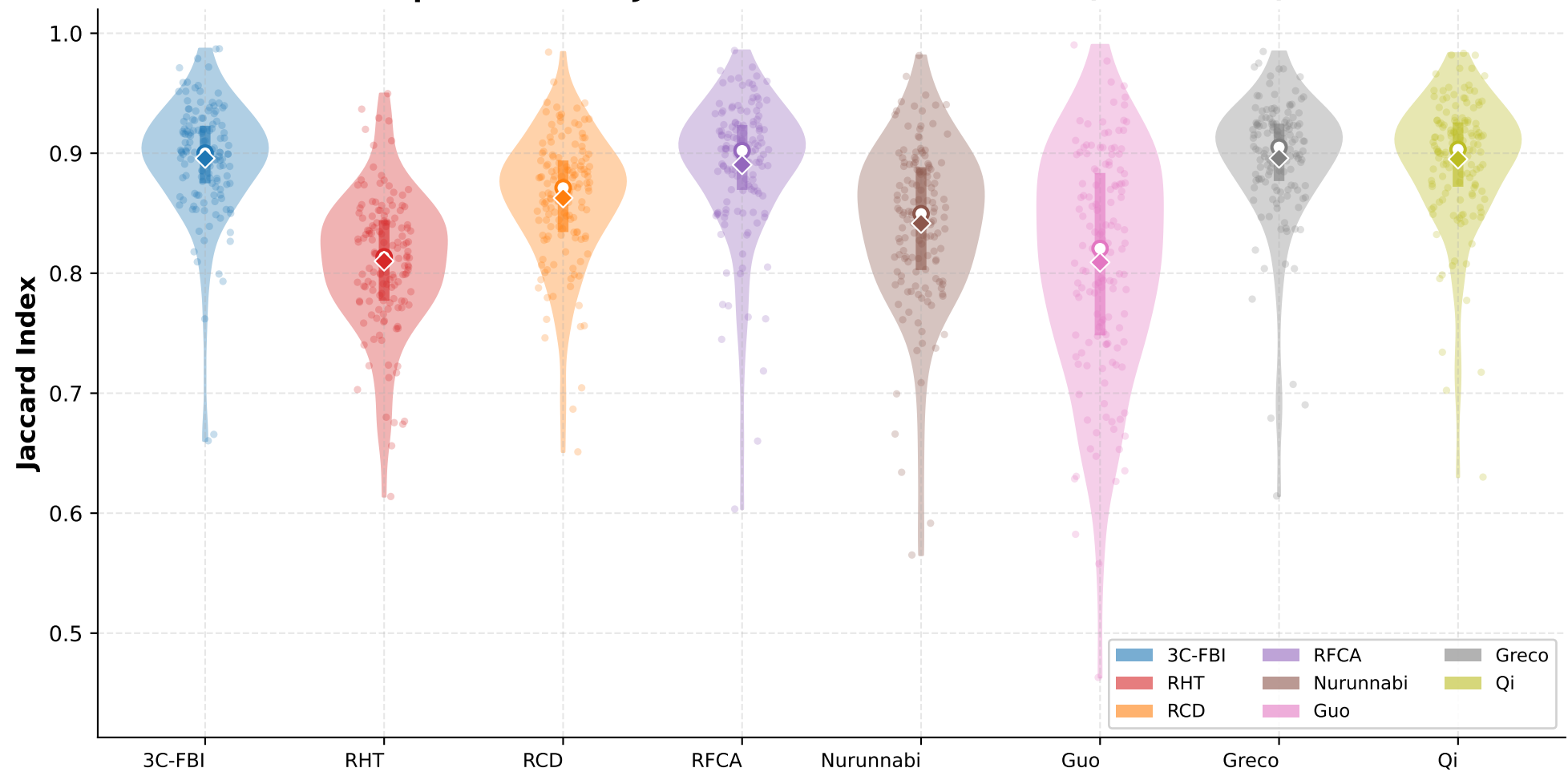
Experiment A — Jaccard Distribution at GL82 (144 frames)
