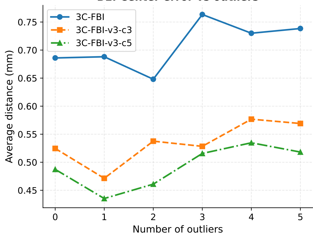
B1: Center error vs outliers
