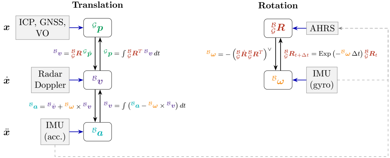
Figure 1: States of the robot. Down arrows derive and up arrows integrate between orders, blue arrows are direct measurements, and dashed arrows are dependencies. Left superscripts give the frame, global \mathcal{G} or body \mathcal{B} , and {}^{\mathcal{B}}_{\mathcal{G}}\mathbf{R} rotates vectors from \mathcal{G} to \mathcal{B} . \text{Exp}(\cdot) maps a rotation vector to SO(3) and (\cdot)^\vee maps a skew-symmetric matrix to its vector.
