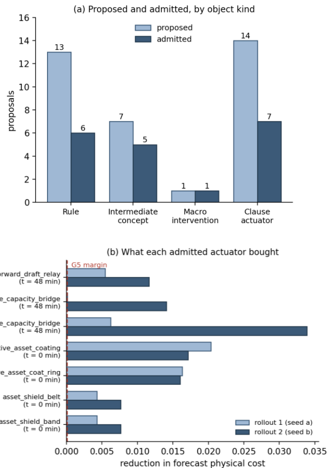
Figure 5.23 Generative products: (a) proposed and admitted by object kind, (b) the forecast cost each admitted actuator removed on the two reseeded rollouts
