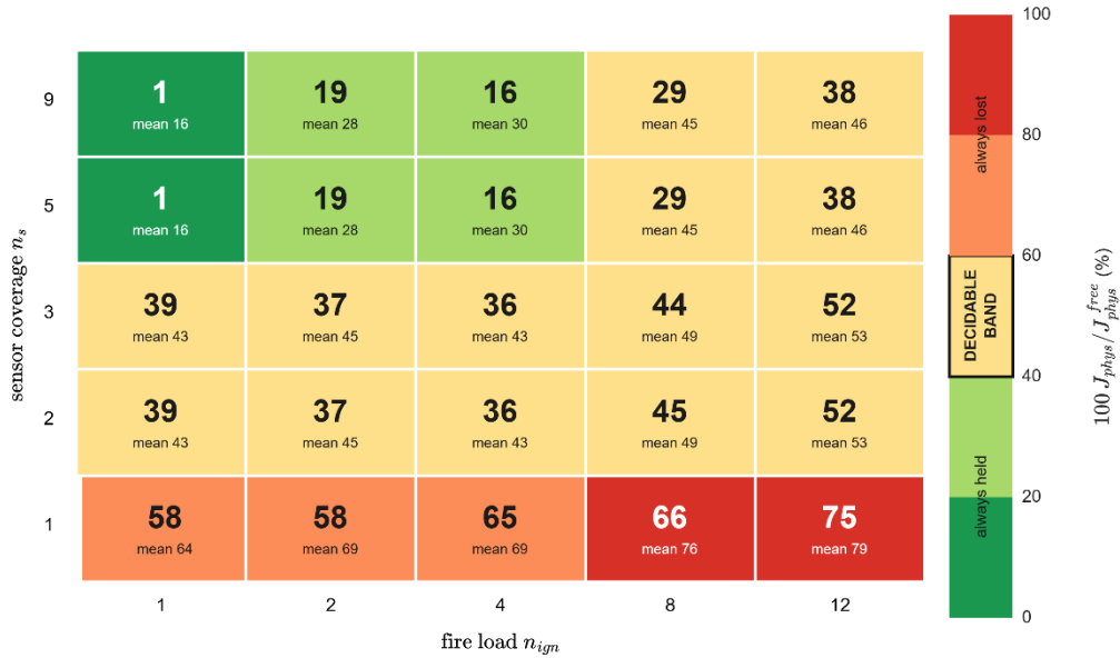
Figure 5.6 The physical cost over ignitions and coverage, pool is 1
