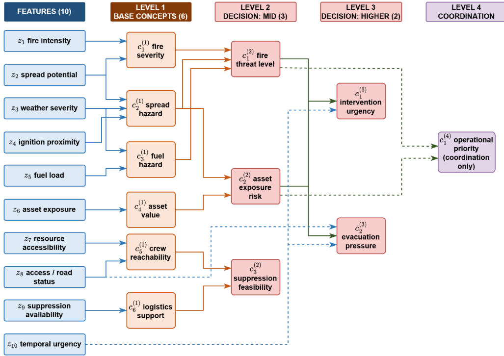
Figure 4.2 Feature-concept hierarchy
