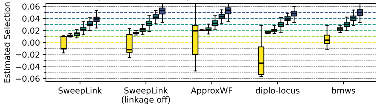
(B) Accuracy of Detected Sweeps across Tools
