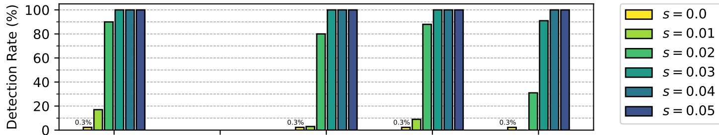
(A) Sweep Detection Performance across Tools
