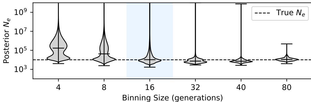
(C) Posterior Uncertainty of N_e across Binning Sizes
