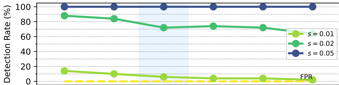
(A) Sweep Detection Performance across Binning Sizes
