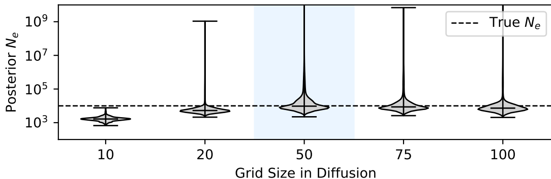
(C) Posterior Uncertainty of N_e across Grid Sizes
