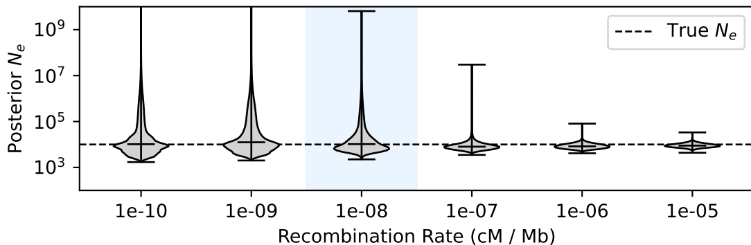
(C) Posterior Uncertainty of N_e across Recombination Rates
