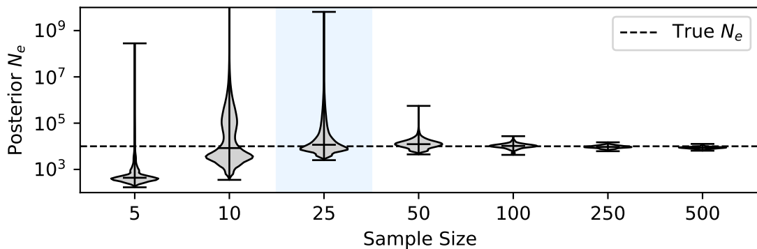
(C) Posterior Uncertainty of N_e across Sample Sizes
