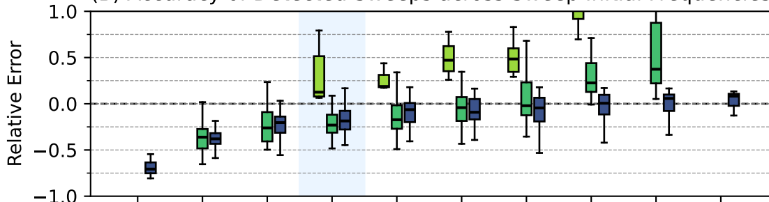
(B) Accuracy of Detected Sweeps across Sweep Initial Frequencies
