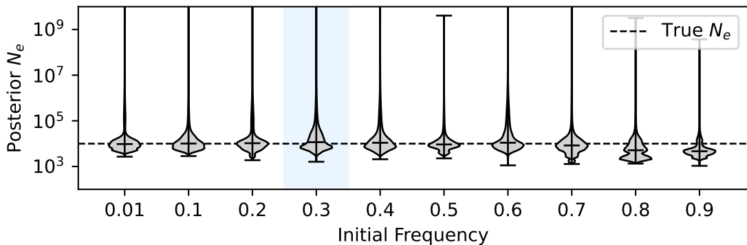
(C) Posterior Uncertainty of N_e across Sweep Initial Frequencies
