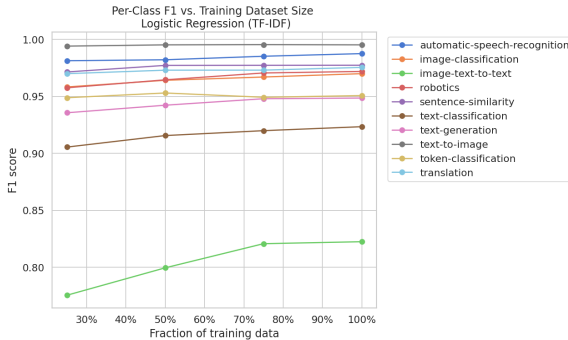
Figure 1: Per Pipeline Tag Class F1 Score from Logistic Regression (TF-IDF) Model
