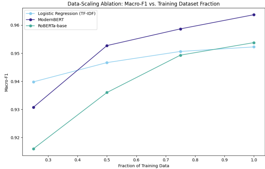
[7] Data-Scaling Ablation Results for Macro-F1 Score per Model vs Training Set Size
