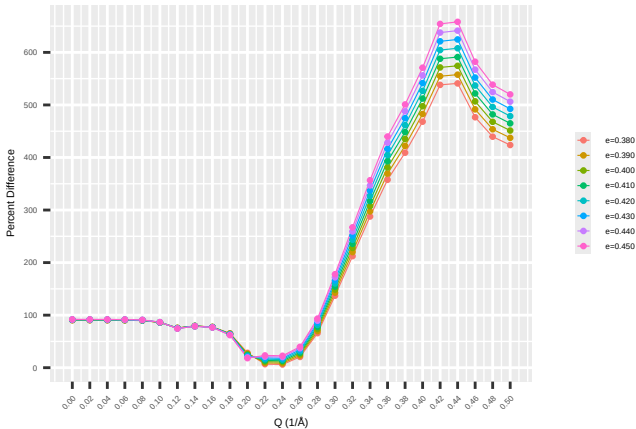
C60BuckyBallHe
