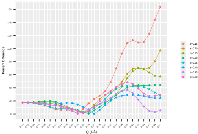
CoiledCoil
