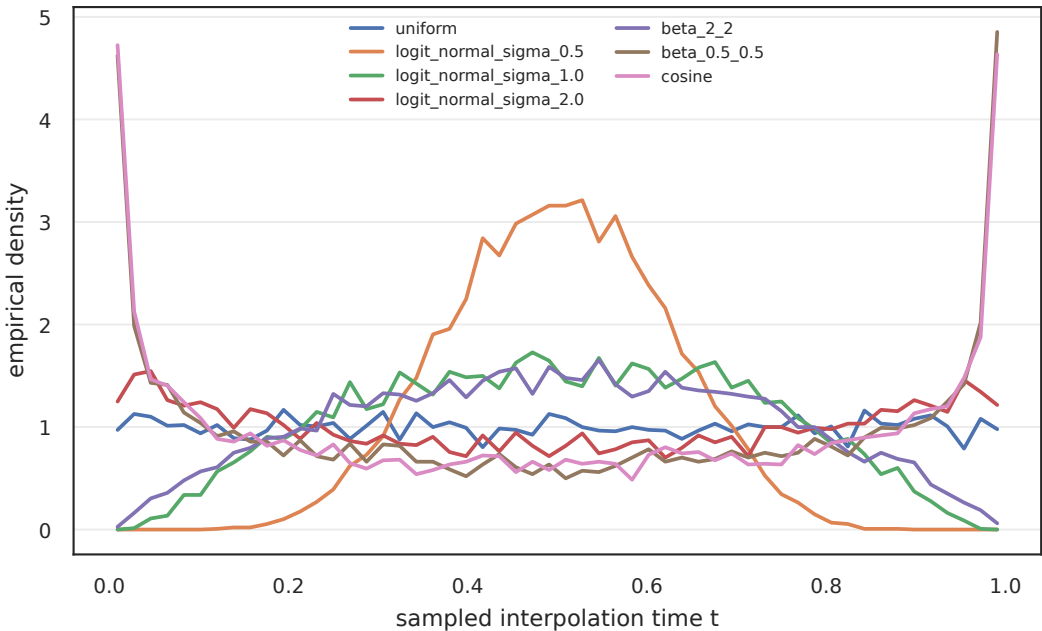
Training-time sampling strategies for CFM
