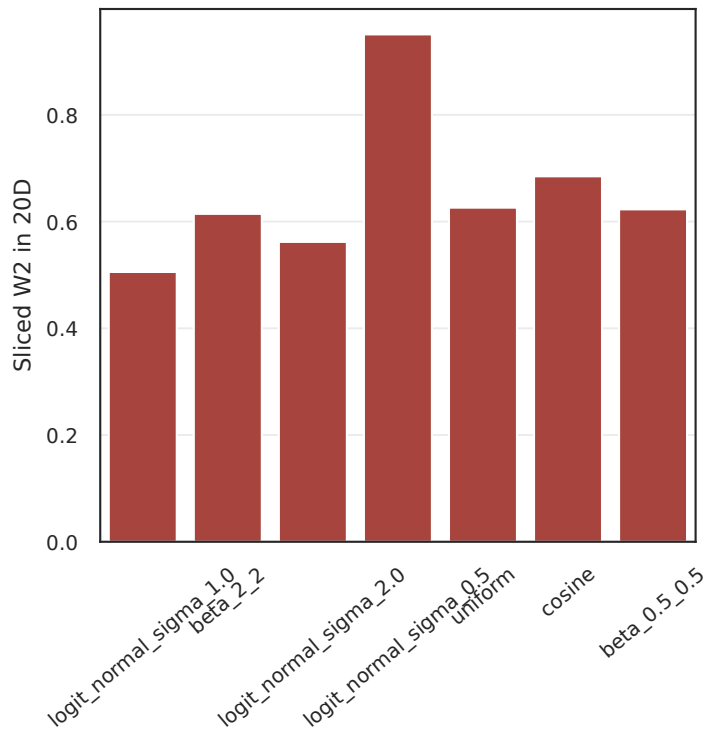
Sliced W2
